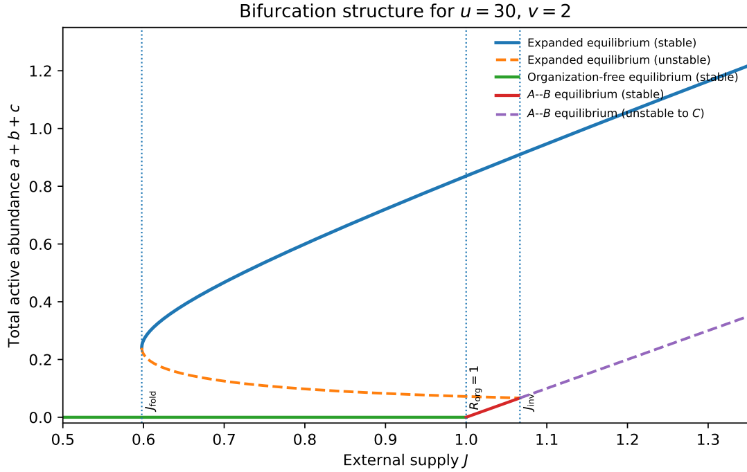
Figure 3: Bifurcation structure for u = 30, v = 2 , plotted as total active abundance a + b + c against external supply J . Solid branches are stable and dashed branches unstable in the stated directions. The expanded branch persists below both the baseline threshold J = 1 and the invasion threshold J_{\text{inv}} , turning at J_{\text{fold}} .
